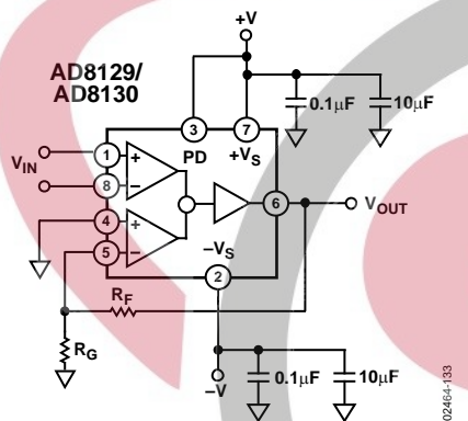
Figure 132. Basic Gain Circuit: V_{OUT} = V_{IN} (1 + R_F/R_G)
