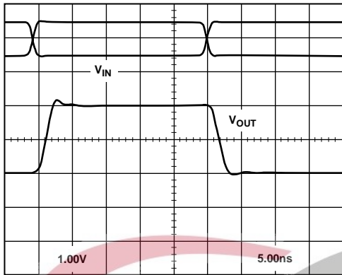
Figure 89. AD8130 Transient Response with +3 V Common-Mode Input
